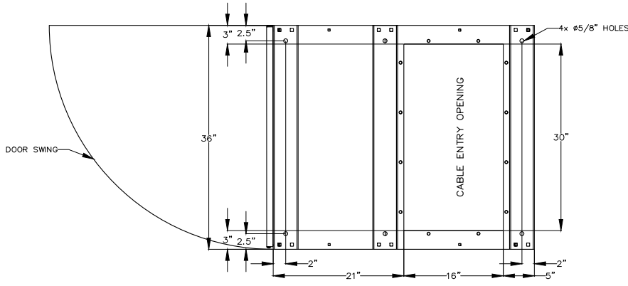
BASE PLAN SECTION B-B
