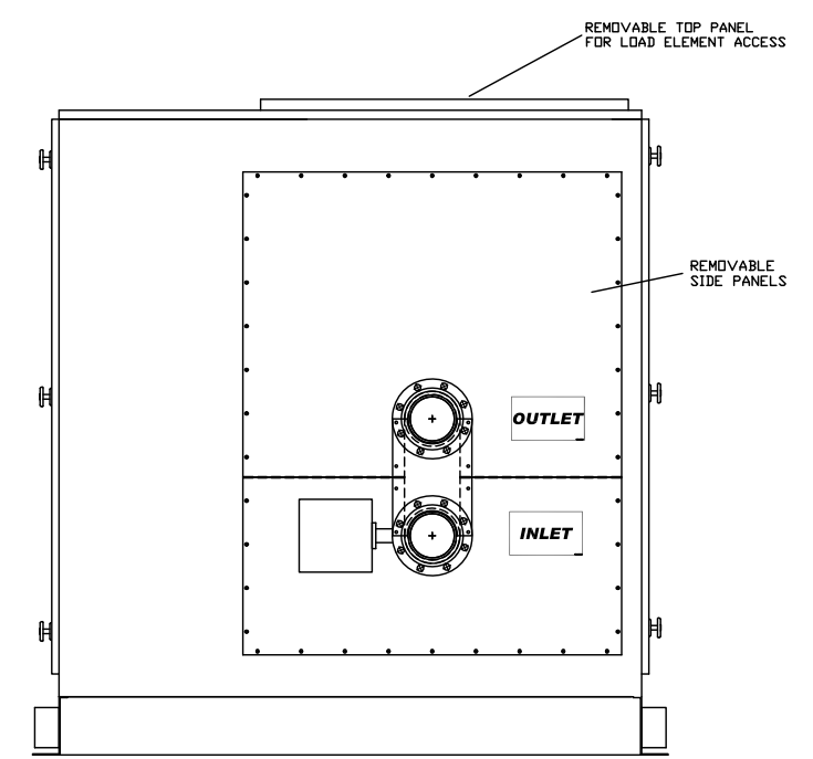
SIDE VIEW
